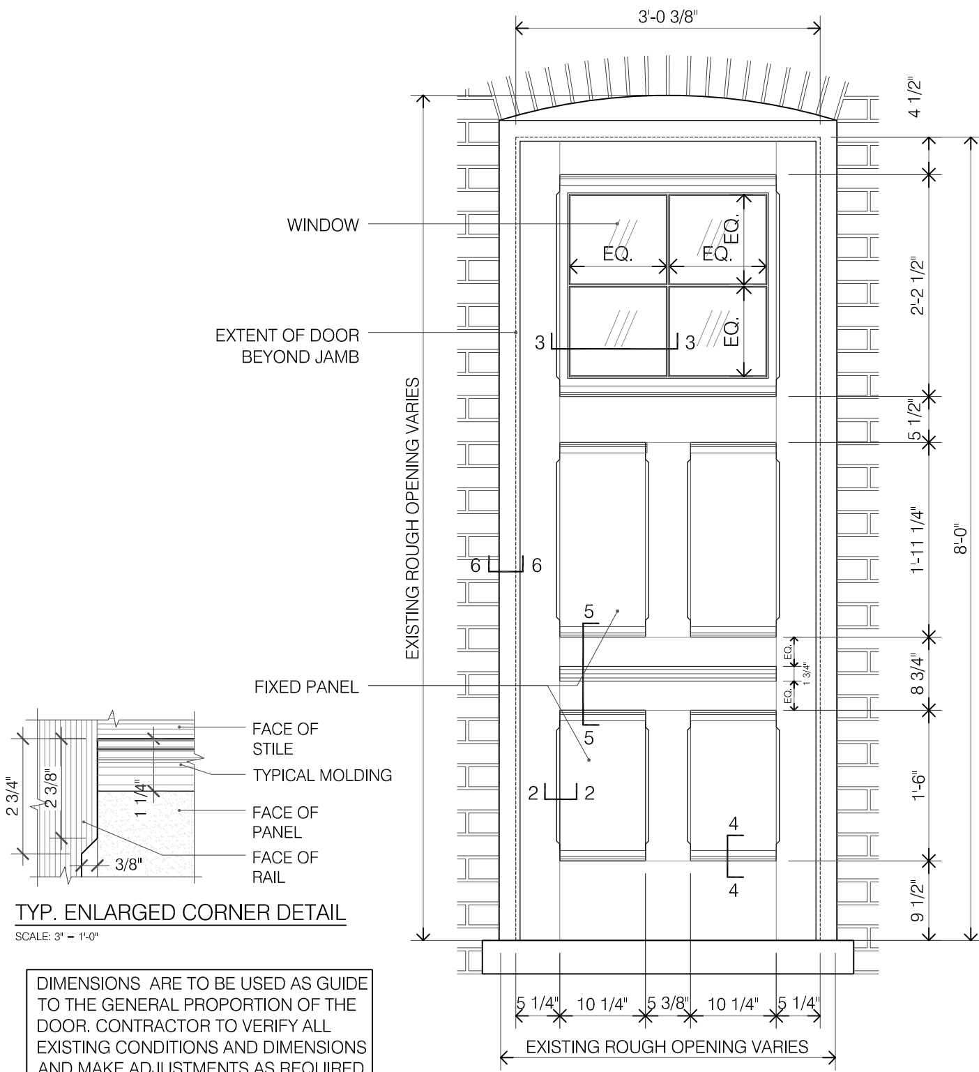
1 EXTERIOR DOOR ELEVATION SCALE: 3/4" = 1'-0"
