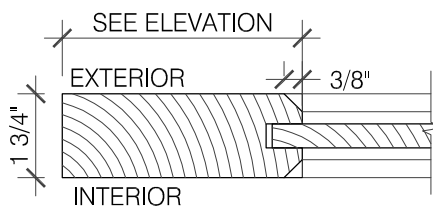
2 SECTION AT STILE AND PANEL SCALE: 3" = 1'-0"
