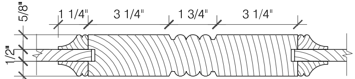
5 DETAIL OF BEADING ON STILE SCALE: 3" = 1'-0"
