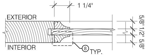
4 SECTION AT RAIL AND PANEL SCALE: 3" = 1'-0"
