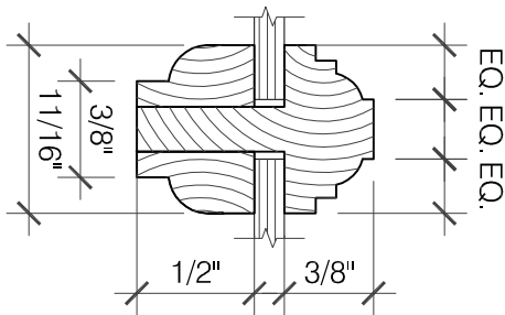
7 GLASS STOP DETAIL SCALE: 1'-0" = 1'-0"
