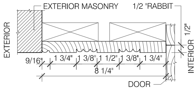
6 SECTION AT BRICK MOLD AND JAMB SCALE: 3" = 1'-0"
