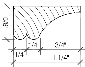
8 PANEL STOP DETAIL SCALE: 1'-0" = 1'-0"
