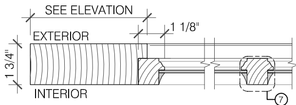
3 SECTION AT STILE/RAIL AND GLASS SCALE: 3" = 1'-0"
