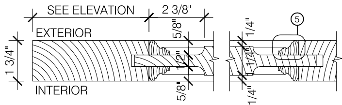
2 SECTION AT STILE AND PANEL SCALE: 3" = 1'-0"
