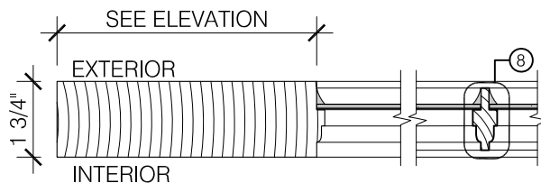
2 SECTION AT STILE/RAIL AND GLASS SCALE: 3" = 1'-0"
