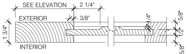
3 SECTION AT STILE AND PANEL SCALE: 3" = 1'-0"
