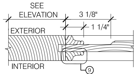
4 SECTION AT RAIL AND PANEL W/STOP SCALE: 3" = 1'-0"
