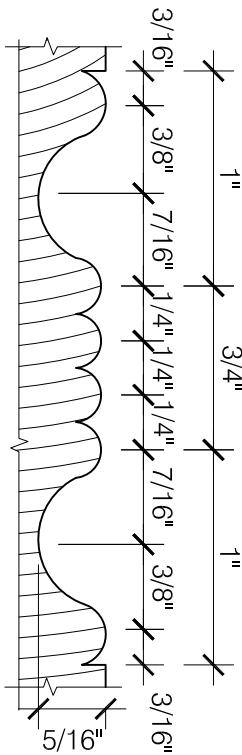
6 DETAIL OF SCROLL WORK IN STILE SCALE: 1'-0" = 1'-0"
