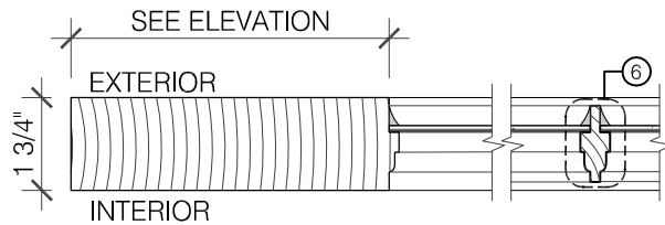
3 SECTION AT STILE/RAIL AND GLASS SCALE: 3" = 1'-0"
