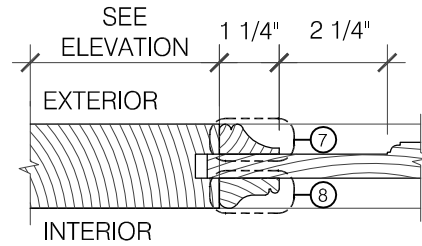
4 SECTION AT RAIL AND PANEL SCALE: 3" = 1'-0"
