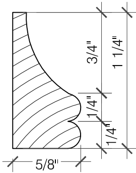
8 PANEL STOP DETAIL SCALE: 1'-0" = 1'-0"
