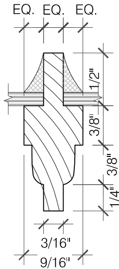
6 GLASS STOP DETAIL SCALE: 1'-0" = 1'-0"
