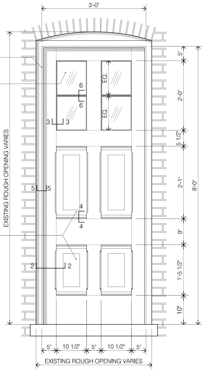
1 EXTERIOR DOOR ELEVATION
