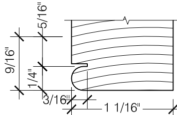
5 TYP. DETAIL OF SCROLL WORK AT BRICK MOLD SCALE: 1'-0" = 1'-0"
