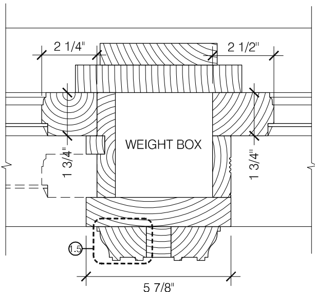
1.4 PLAN DETAIL OF MULLION SCALE: 3' = 1'-0"
