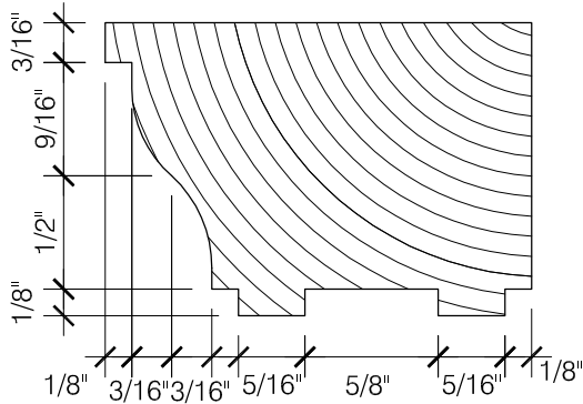
1.5 PLAN DETAIL OF MULLION SCALE: 1'-0" = 1'-0"
