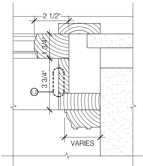
1.3 JAMB/HEAD DETAIL AT SIDE LIGHT SCALE: 3' = 1'-0"
