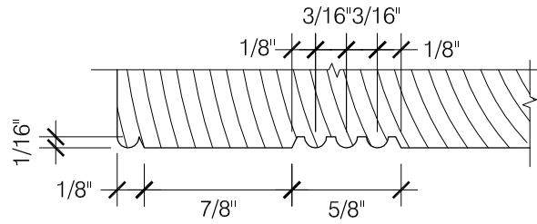
1.2 DETAIL OF SCROLL WORK AT SIDE LIGHT SCALE: 1'-0" = 1'-0"
